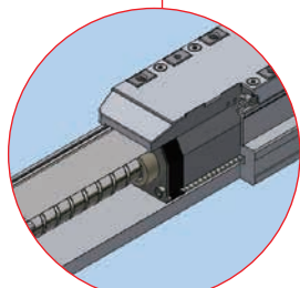
內嵌型直線滾珠滑軌 Built-in linear circular guideway
